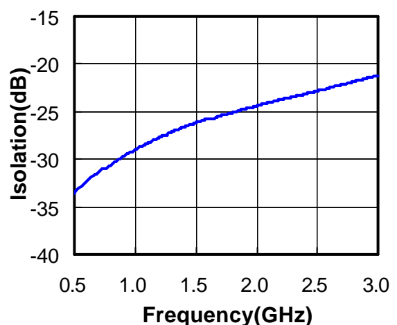
RF1 RF2 Isolation vs. Frequency
